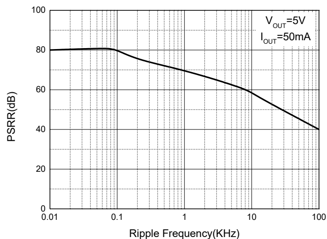
PSRR vs. Frequency ( V_{IN}=6V+aV_{P-PAC} )
